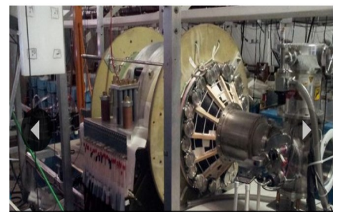
The fusion driven rocket test chamber at the UW Plasma Dynamics Lab in Redmond. The green vacuum chamber is surrounded by two large, high-strength aluminum magnets. These magnets are powered by energy-storage capacitors through the many cables (University of Washington, MSNW)
